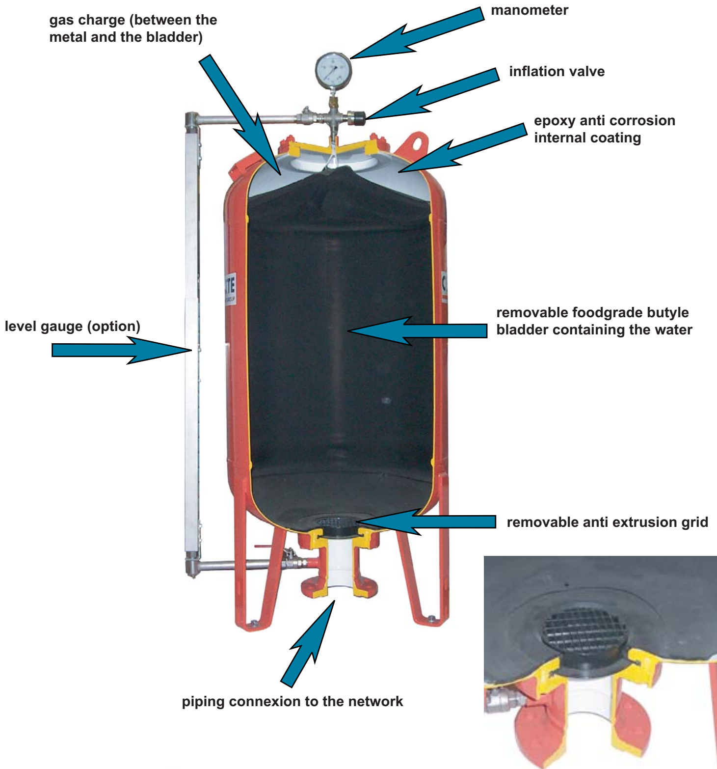
Foodgrade butyle bladder surge vessel
